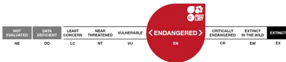
Fig. 1. The IUCN Red List Categories: NE ( Non-evaluated ) to EX ( Extinct ). https://www.iucn.org/resources/conservation-tools/iucn-red-list-threatened-species
